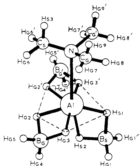
Figure 13. The structure by x-ray diffraction of (\text{CH}_3)_3\text{NAl}(\text{BH}_4)_3 at -160^\circ\text{C} from ref 169.
