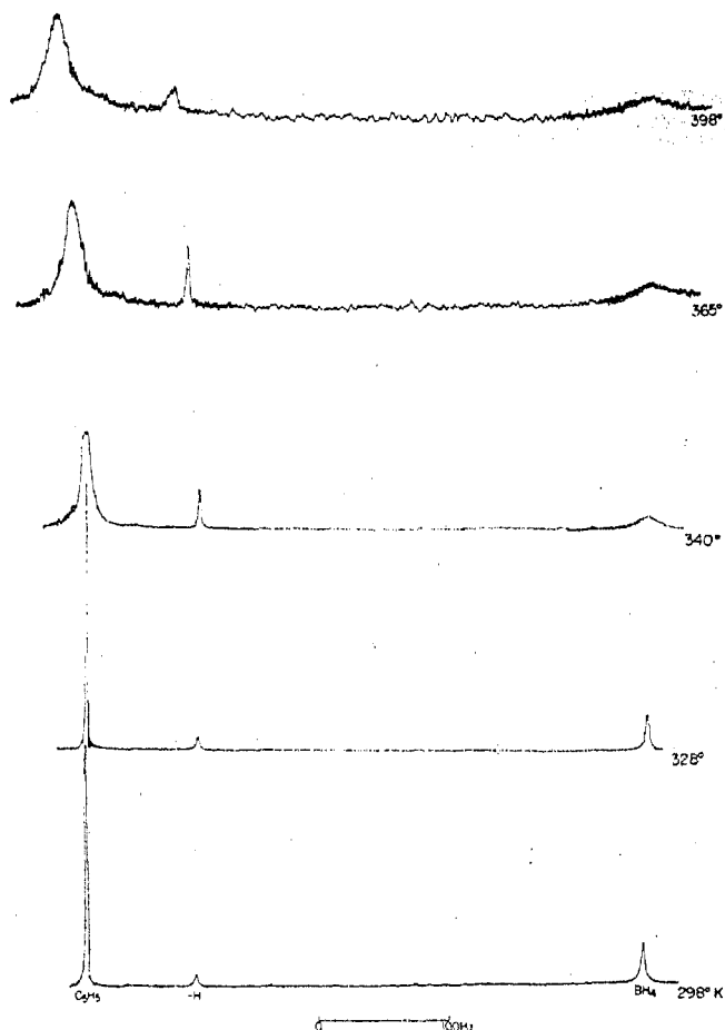
Figure 11. Variable-temperature 90-MHz ^1\text{H} NMR spectra of (\eta^5\text{-C}_5\text{H}_5)_2\text{Zr}(\text{H})\text{BH}_4 in toluene- d_8 with broad-band decoupling of ^{11}\text{B} (ref 149).
