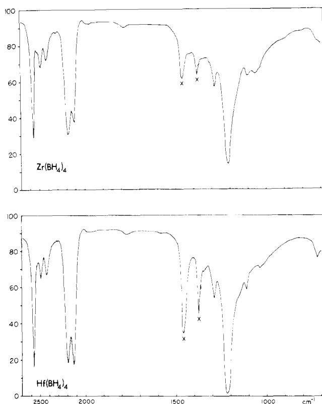
Figure 3. Infrared spectra of Zr(BH_4)_4 and Hf(BH_4)_4 as solutions in Nujol. The sharp bands due to Nujol are marked X (ref 77).
