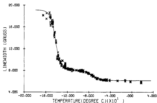
Figure 10. The temperature dependence of the ^1\text{H} NMR line width of a polycrystalline sample of \text{Hf}(\text{BH}_4)_4 (from ref 139).
